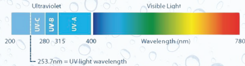
Electromagnetic Spectrum
